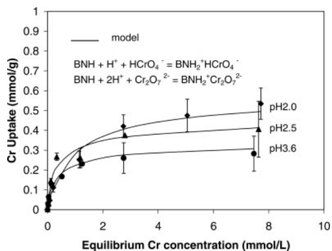
Figure 1. Modeling the effect of pH on chromium (VI) biosorption by AWCS.
