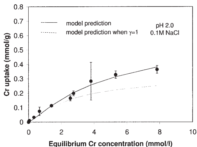
Figure 2. Model prediction of the ionic strength effect on chromium biosorption by AWCS.
